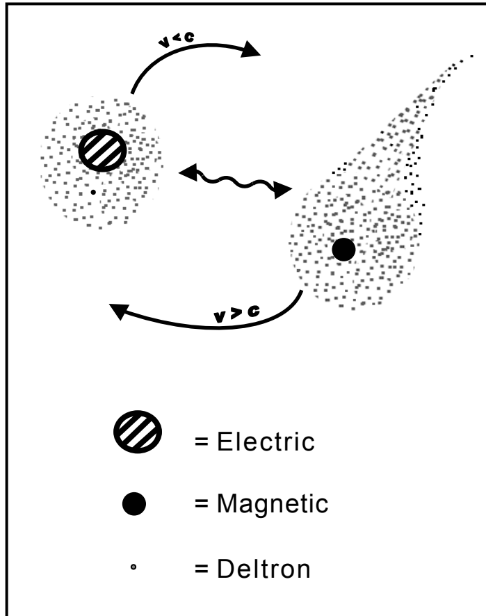
Figure 7. Illustration of how deltron sheaths can allow faster than light particles to interact with slower than light particles.
