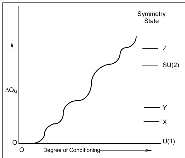
Figure 2. Schematic illustration of free energy change, \Delta Q_G , from the ground symmetry state, U(1), as the degree of locale conditioning increases.
