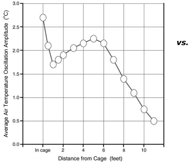
Figure 3. Composite amplitude distance plot for air T- oscillations.
